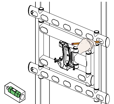
Right-Hand Swingout Arm Orientation
