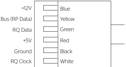
Standard RJ-22 can be used in place of RJ-14 cable
