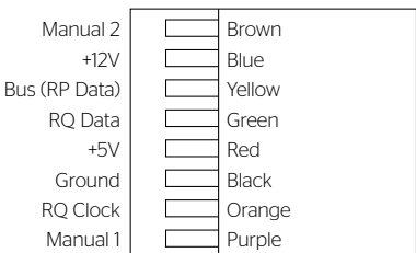
RJ-45 Pin-Outs (Tab Is Facing Down)
