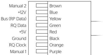
RJ-45 Pin-Outs (Tab Is Facing Up)
