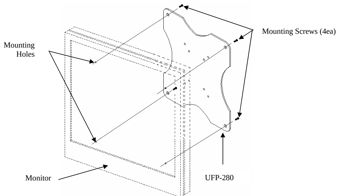
Figure 1. UFP-280 Installation
