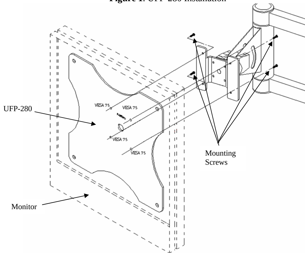
Figure 2. Mount Installation
